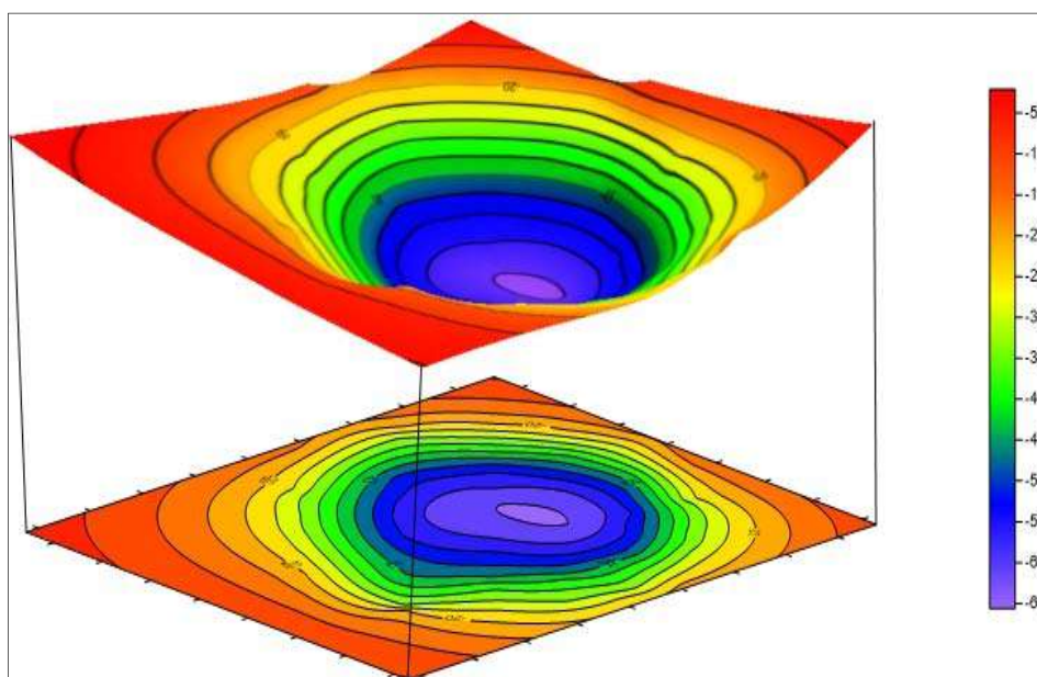
Fig. 10. Combination of 2D and 3D maps of the vertical component of the gravity force ( V_z ) of the Yevlakh-Agjabadi Basin (in milligals)
