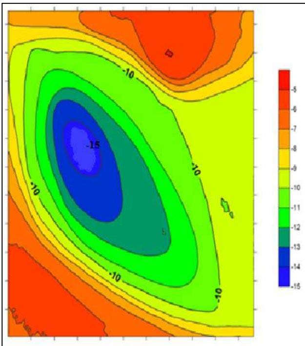
Fig.4. Structural map of the crystalline basement (in km) of the Yevlakh-Agjabadi basin developed using the SURFER program
